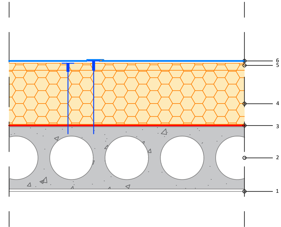
260 mm MW ( \lambda = 0.038 \text{ W/mK} )
