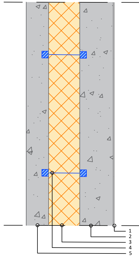
140 mm IP PIR 022 ( \lambda = 0.022 W/mK)
