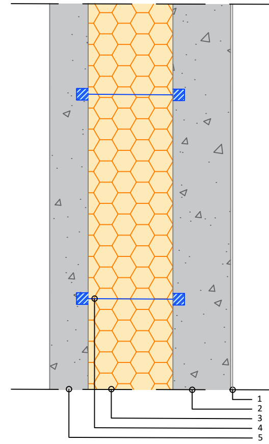
220 mm MW ( \lambda = 0.035 W/mK)
