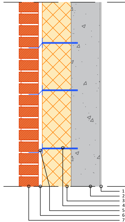
150 mm Powerwall Pro ( \lambda = 0.026 \text{ W/mK} )
