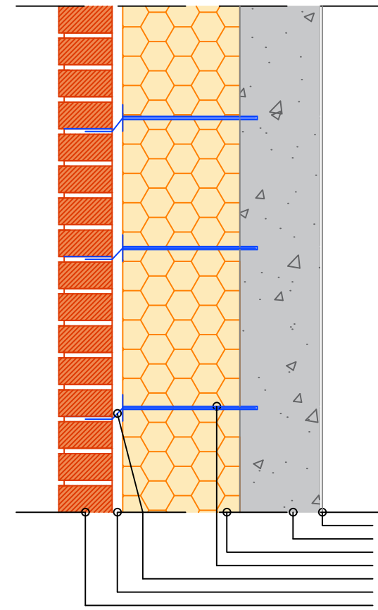
220 mm MW ( \lambda = 0.035 \text{ W/mK} )
